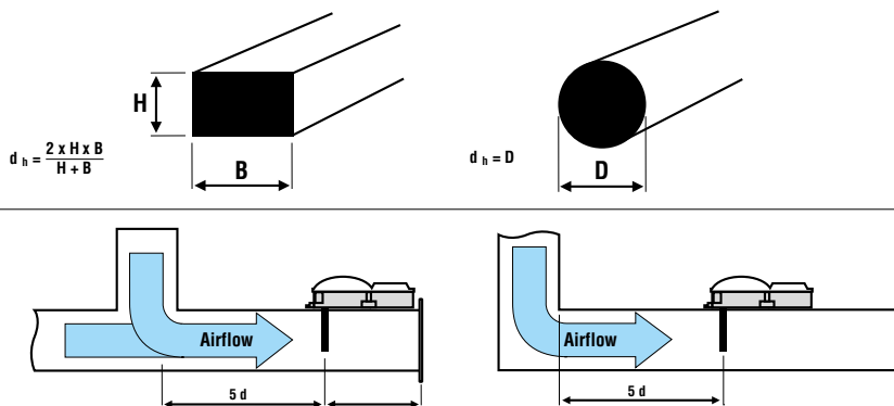
Application example with detector
